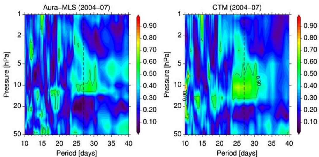
Figure 3: Coherence between solar UV flux and time series of stratospheric tropical ozone (50-1 hPa) (left) measured by Aura MLS and (right) simulated by the LMDz-Reprobus model in its guided configuration (meaning that the dynamic is recalled with the meteorological re-analysis) over the period 2004-2007. Observations and results of models show a coherent and significant ozone response to the UV solar flux which seems centered on a period of 27 days at 10 hPa (~ 30 km). Credits: CNRS.
