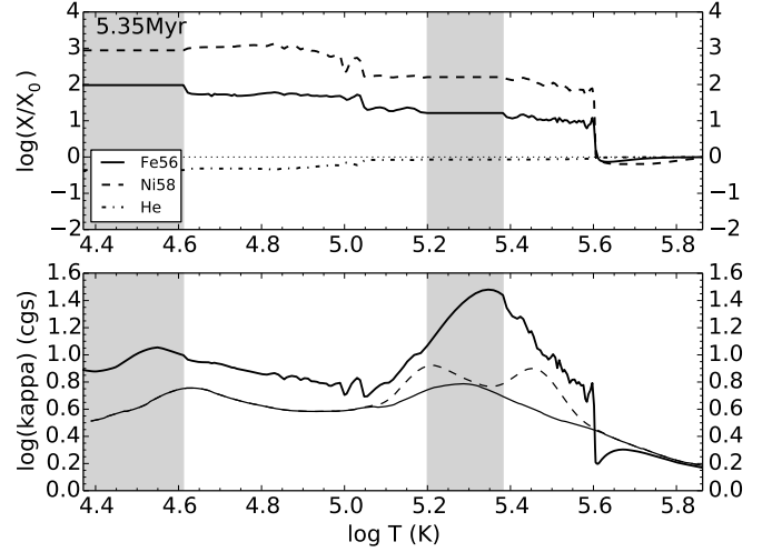
Fig. 3. Same as Fig. 2 for a model with fingering mixing.
