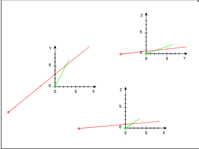
Fig. 1: The geometry of the encounter of 'Oumuamua with the star G 108-21 0.2 Myr ago. Depicted is 0.3 Myr of their motion.
