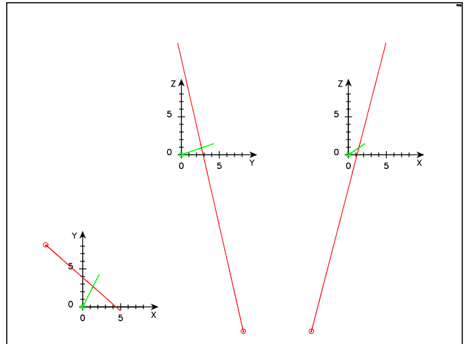
Fig. 4: The geometry of the encounter of 'Oumuamua with the star HIP 3757 118 kyr ago. 186 kyr of motion of these bodies is shown here.
