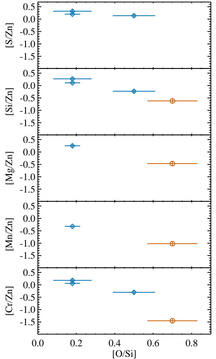
Fig. 2. Same as Fig. 1, but using [\text{O}/\text{Si}] as a proxy for the dust content.
