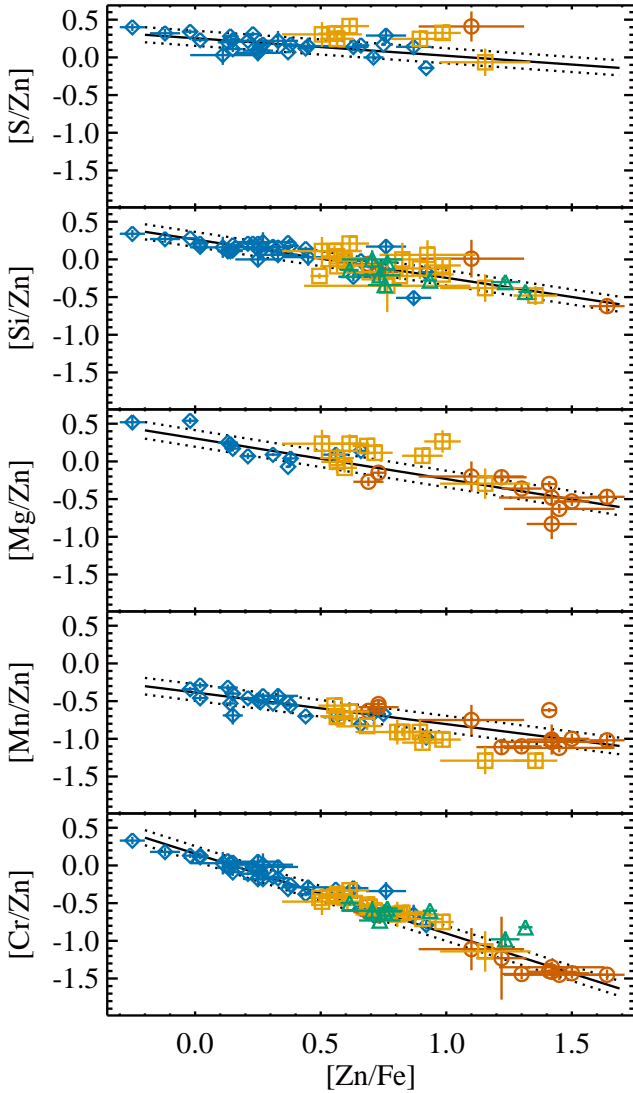
Fig. 1. Relative abundances observed in the Galaxy (orange circles, Jenkins 2009), SMC (yellow squares, Tchernyshyov et al. 2015; Jenkins & Wallerstein 2017), LMC (green triangles, Tchernyshyov et al. 2015), and DLAs (blue diamonds, De Cia et al. 2016). The [\text{Zn}/\text{Fe}] is a proxy for the dust content, while the [X/\text{Zn}] traces the dust depletion of element X . The solid lines are from De Cia et al. (2016) and were derived from a linear fit to the Galactic and DLA data, not including the Magellanic Clouds, where the intrinsic scatter is marked by the dotted lines.
