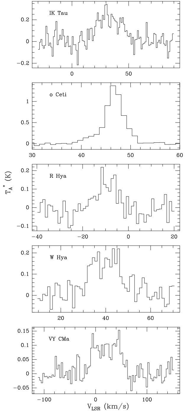
Fig. 3. Spectra of the J = 6-5 transition of ^{13}\text{CO} at 661 GHz toward five stars in our sample, plotted at 1.1 \text{km s}^{-1} resolution (3.0 \text{km s}^{-1} for VY CMa). The antenna temperature is for outside the atmosphere. See Sect. 2.3 for Jy to K conversion at the time of the observations.
