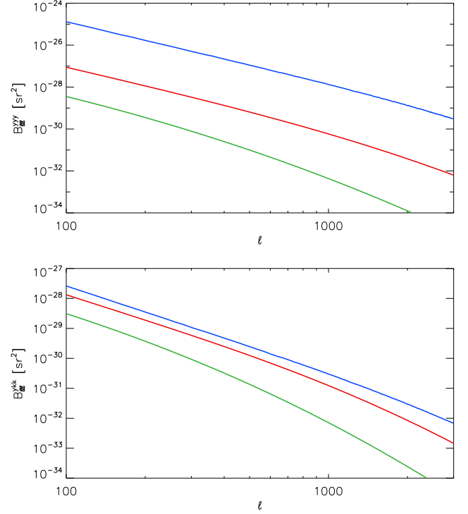
Fig. 2. tSZ (top panel) and tSZ-kSZ-kSZ (bottom panel) bispectra 1-halo term (blue line), 2-halo term (red line), and 3-halo term (green line).
