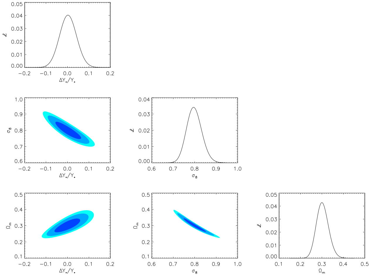
Fig. 4. Likelihood for combined tSZ power spectrum, bispectrum, and tSZ-kSZ-kSZ bispectrum as a function of Y_* , \sigma_8 , and \Omega_m . Dark blue, blue, and light blue contours indicate the 1, 2, and 3\sigma levels.
