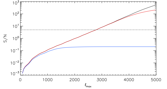
Fig. 3. Cumulative S/N for the tSZ-kSZ-kSZ bispectrum as a function of \ell for a cosmic-variance-limited experiment (black line), the Planck experiment (blue line), and a CORe+ like experiment (red line). The dashed line shows the 5\sigma level.
