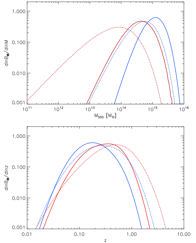
Fig. 1. Power density as a function of M_{500} (top panel) and redshift ( bottom panel ) for the tSZ power spectrum (dotted blue line), the tSZ bispectrum (solid blue line), the kSZ power spectrum (dotted red line), and the tSZ-kSZ-kSZ bispectrum (solid red line).
