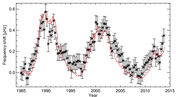
Fig. 3. Frequency shifts of solar p -modes from BiSON data with 1\sigma error bars (black). The seven month boxcar smoothed monthly sunspot number is shown in red. Source of the sunspot number: WDC-SILSO, Royal Observatory of Belgium, Brussels.
