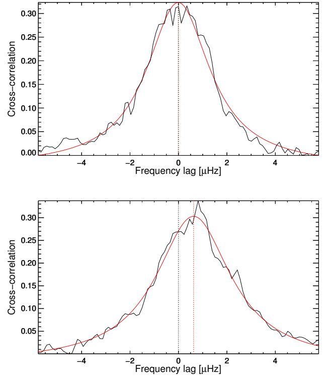
Fig. 2. Top panel: cross-correlation between the part of interest of the LS-periodograms of two realisations of the first segment of KIC 8006161 (black). The Lorentzian fit to the cross-correlation is shown in red. The dotted black vertical line marks zero frequency lag, the dashed red line marks the centre of the fitted Lorentzian. Bottom panel: same as in the top panel, but for the cross-correlation between a realisation of the first and one of the nineteenth segment.
