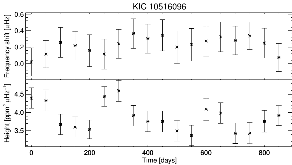
Fig. B.18. Frequency shifts ( top half ) and height of the p -mode envelope ( bottom half ) for KIC 10516096 as a function of time.
