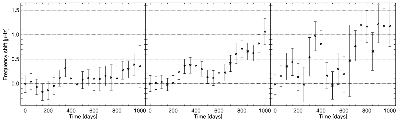
Fig. 8. Frequency shifts of KIC 8006161 for three frequency ranges as a function of time: 2800–3300 \mu\text{Hz} (left panel), 3300–3800 \mu\text{Hz} (middle panel), and 3800–4400 \mu\text{Hz} (right panel).
