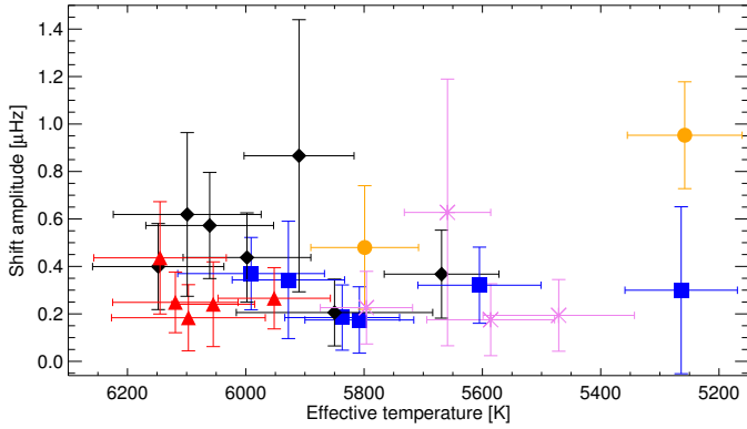
Fig. 4. Measured shift amplitudes as a function of effective temperature. Colour and symbol coding: black diamonds represent stars younger than 4 Gyr, red triangles are stars between 4–5 Gyr, orange circles between 5–6 Gyr, blue squares between 6–7 Gyr, and purple asterisks are stars older than 7 Gyr.
