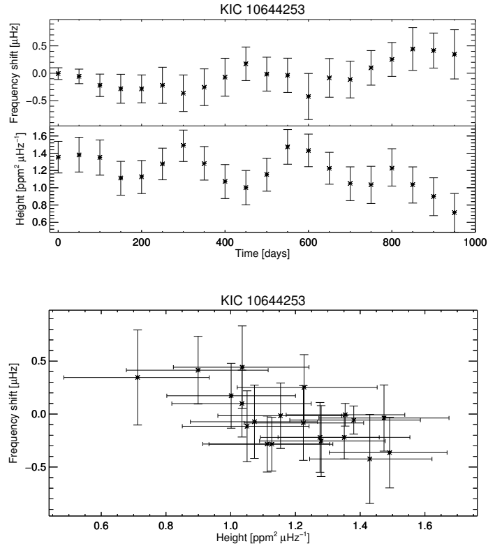
Fig. 9. Top panel: frequency shifts for KIC 10644253 for the frequency range between 2450–3350 \mu\text{Hz} (top half) and height of the p -mode envelope of KIC 10644253 as a function of time (bottom half). Bottom panel: frequency shift as a function of height of the p -mode envelope.
