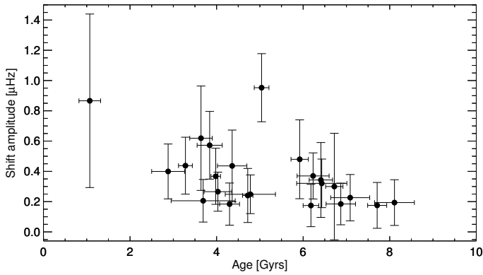
Fig. 5. Measured shift amplitudes as a function of stellar age.
