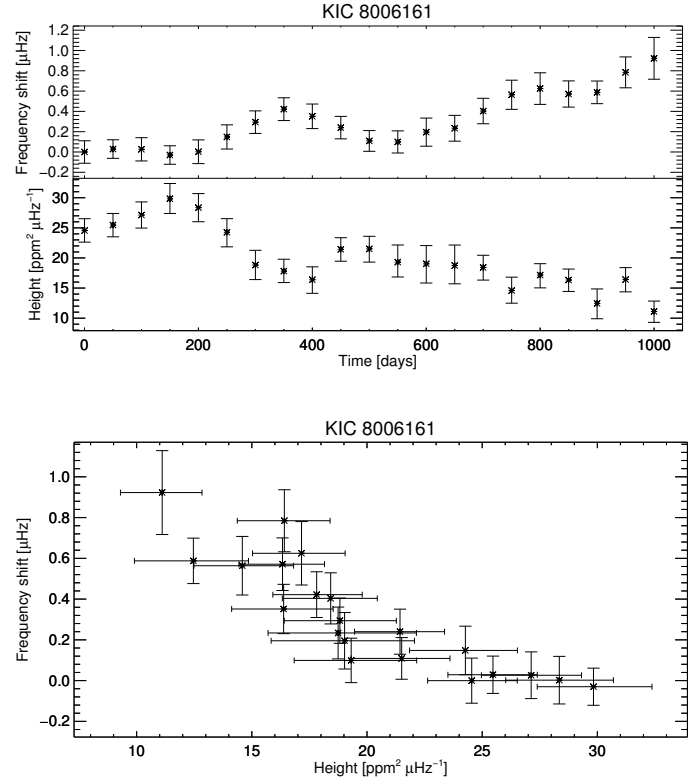
Fig. 7. Top panel: frequency shifts for KIC 8006161 for the frequency range between 2800–4400 \mu\text{Hz} (top half) and height of the p -mode envelope of KIC 8006161 (bottom half) as a function of time. Bottom panel: frequency shift as a function of height of the p -mode envelope.
